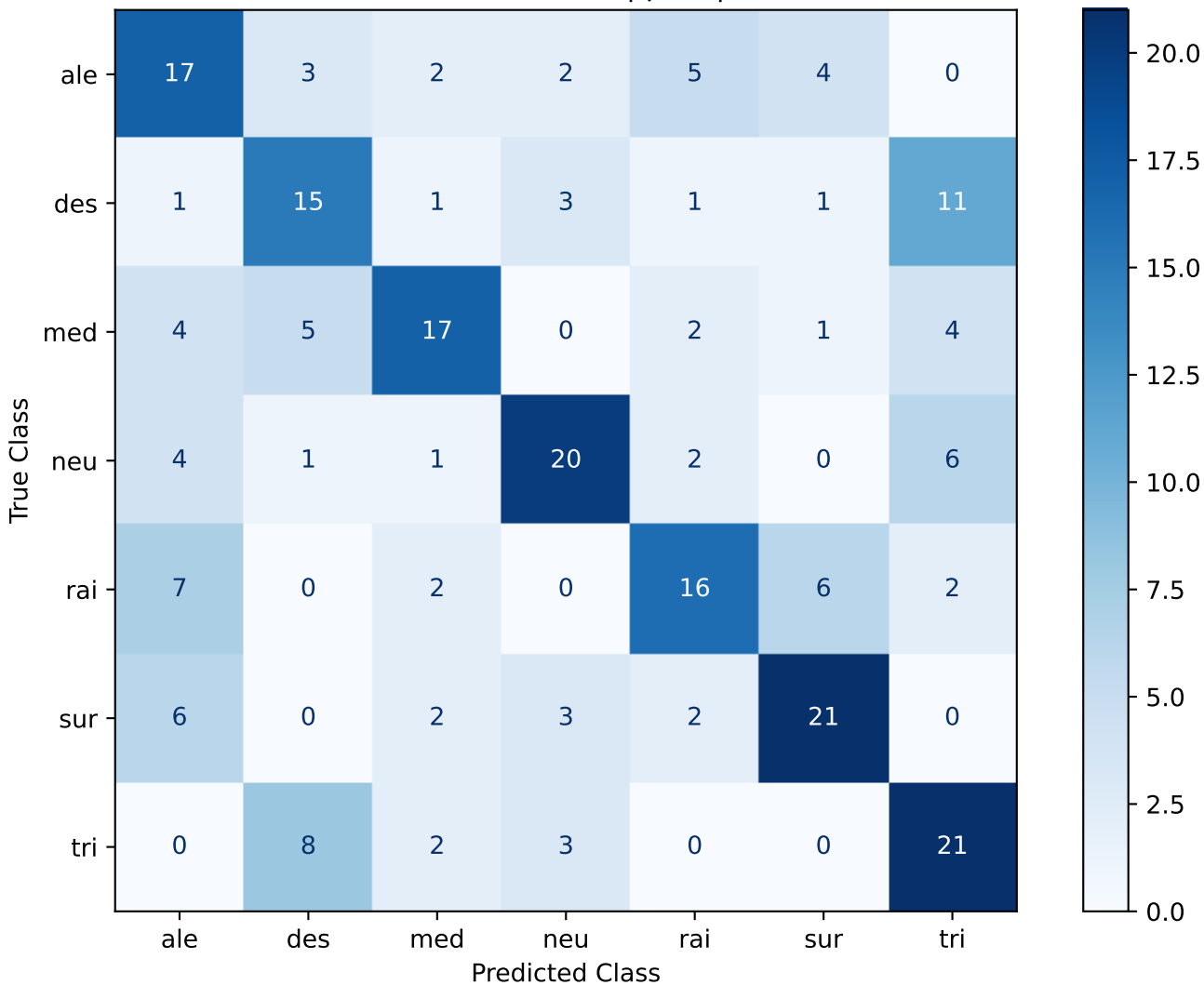
Confusion Matrix - SVC | pAA | Seed 97
