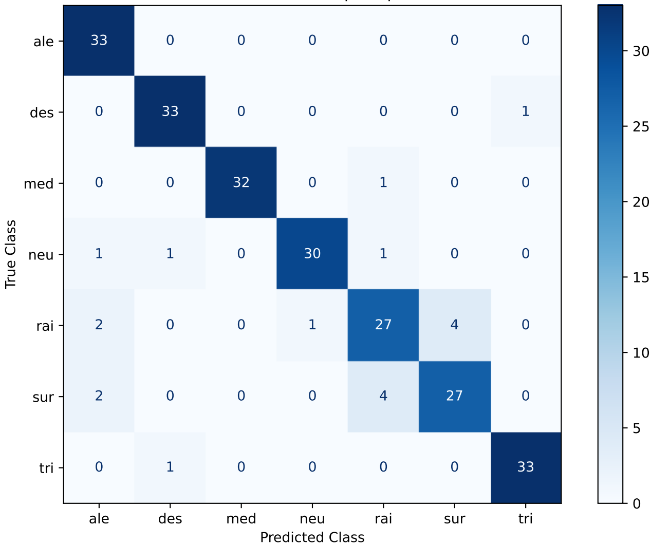
Confusion Matrix - SVC | trill | Seed 123
