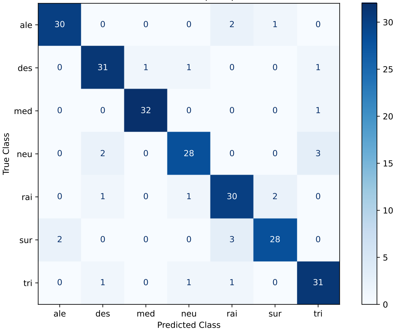
Confusion Matrix - SVC | trill | Seed 2025
