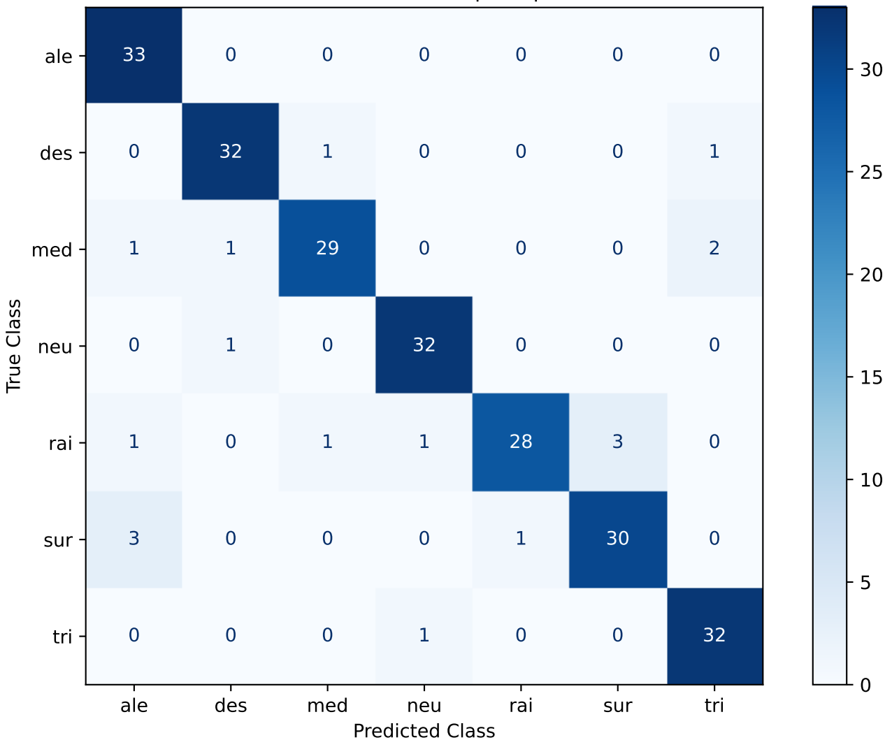
Confusion Matrix - SVC | trill | Seed 42
