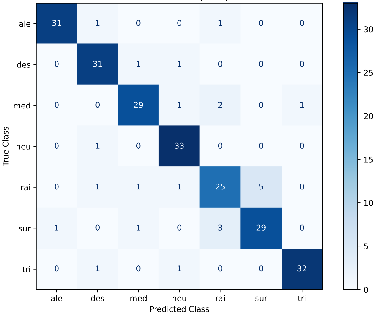
Confusion Matrix - SVC | trill | Seed 97
