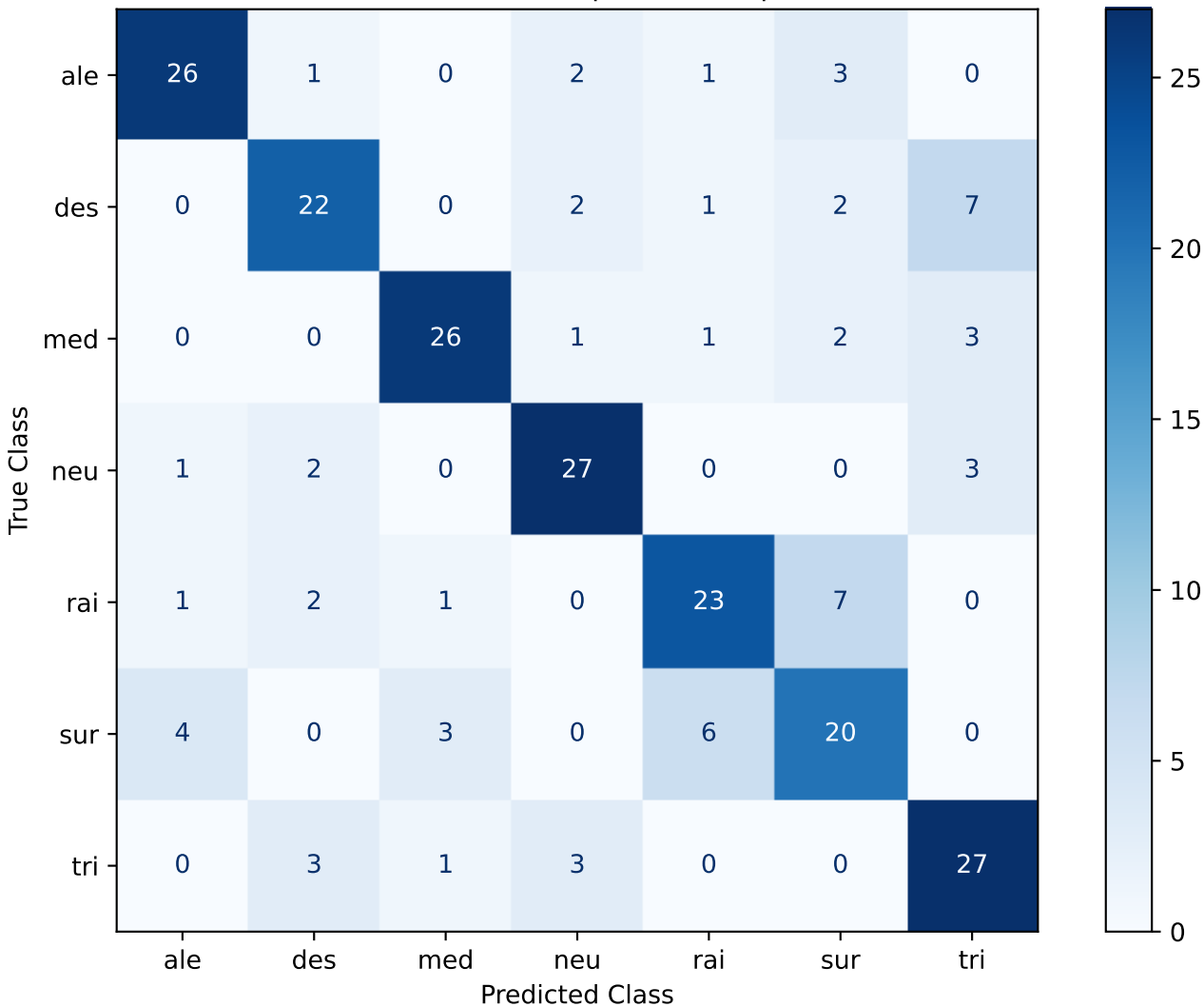
Confusion Matrix - SVC | trillsson5 | Seed 123
