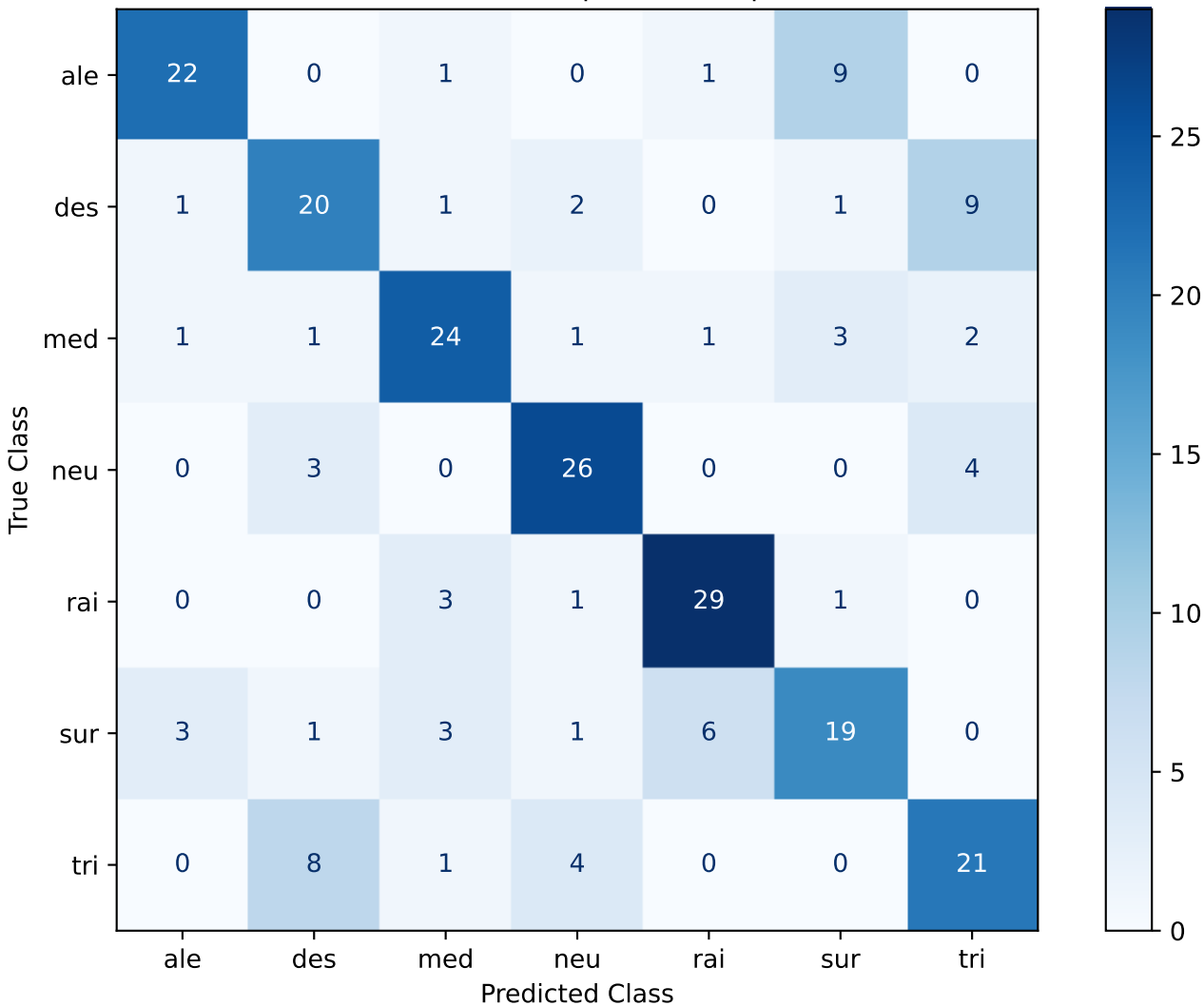
Confusion Matrix - SVC | trillsson5 | Seed 2025
