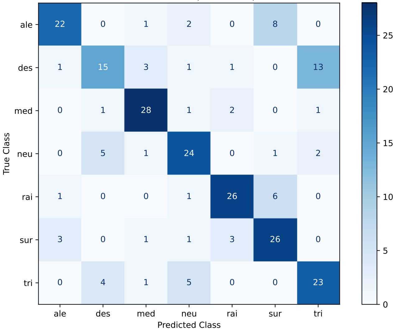
Confusion Matrix - SVC | trillsson5 | Seed 42
