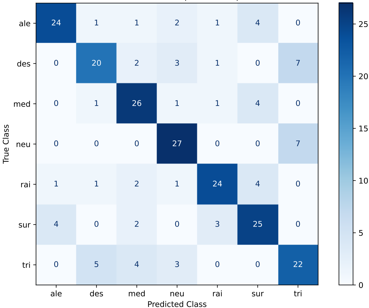
Confusion Matrix - SVC | trillsson5 | Seed 97
