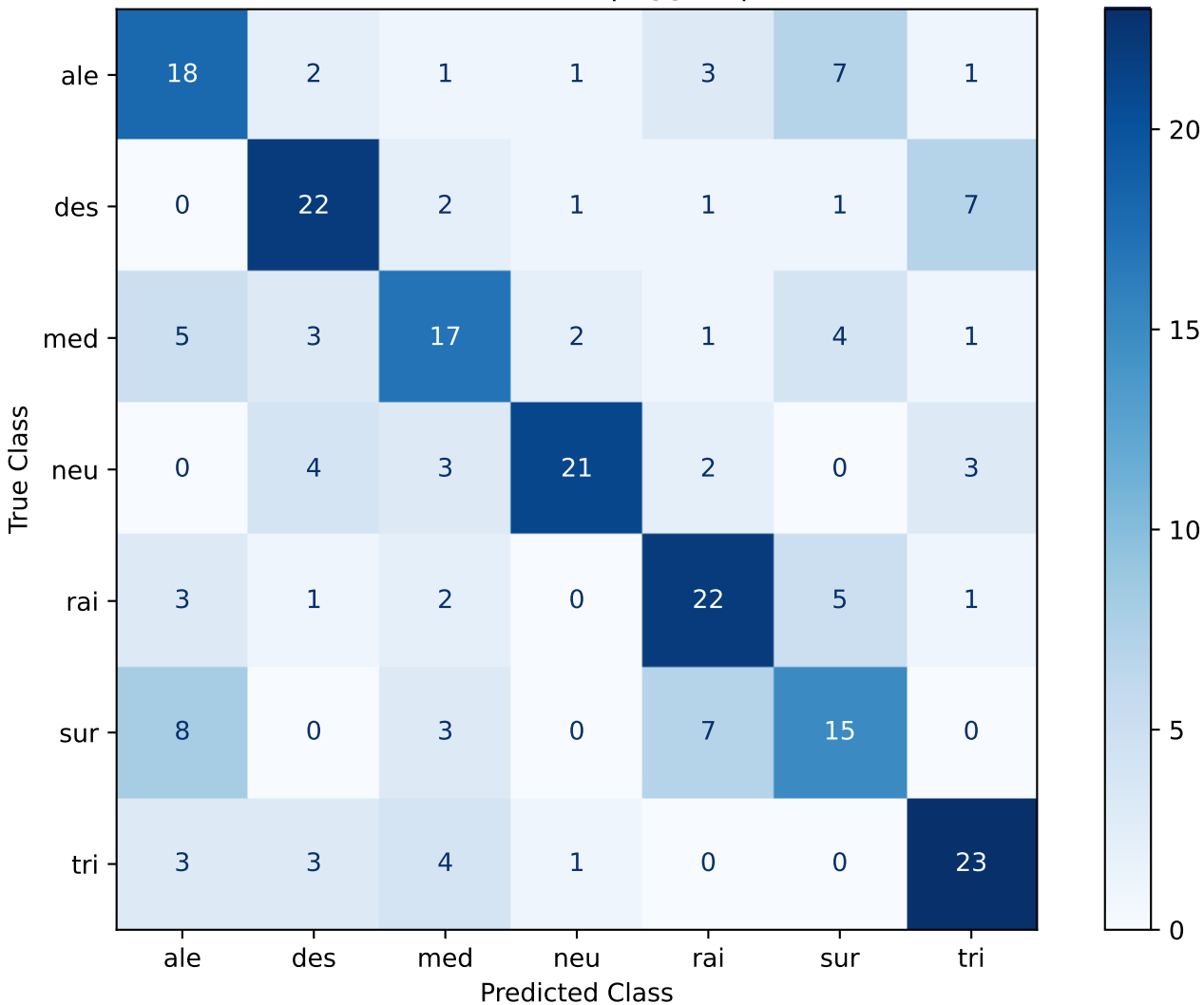
Confusion Matrix - SVC | vggish | Seed 123
