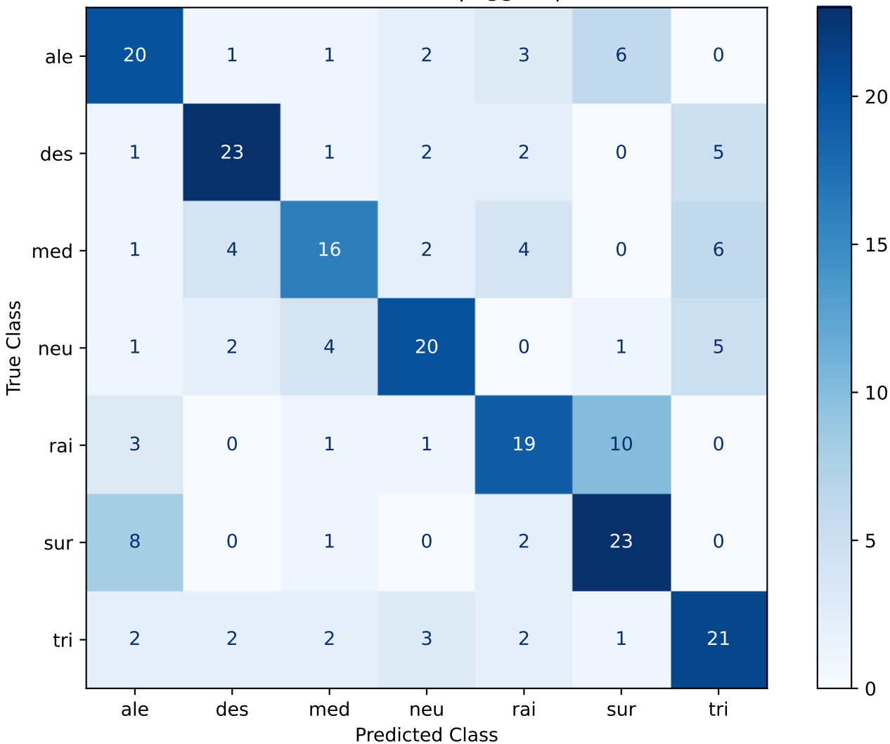
Confusion Matrix - SVC | vggish | Seed 42
