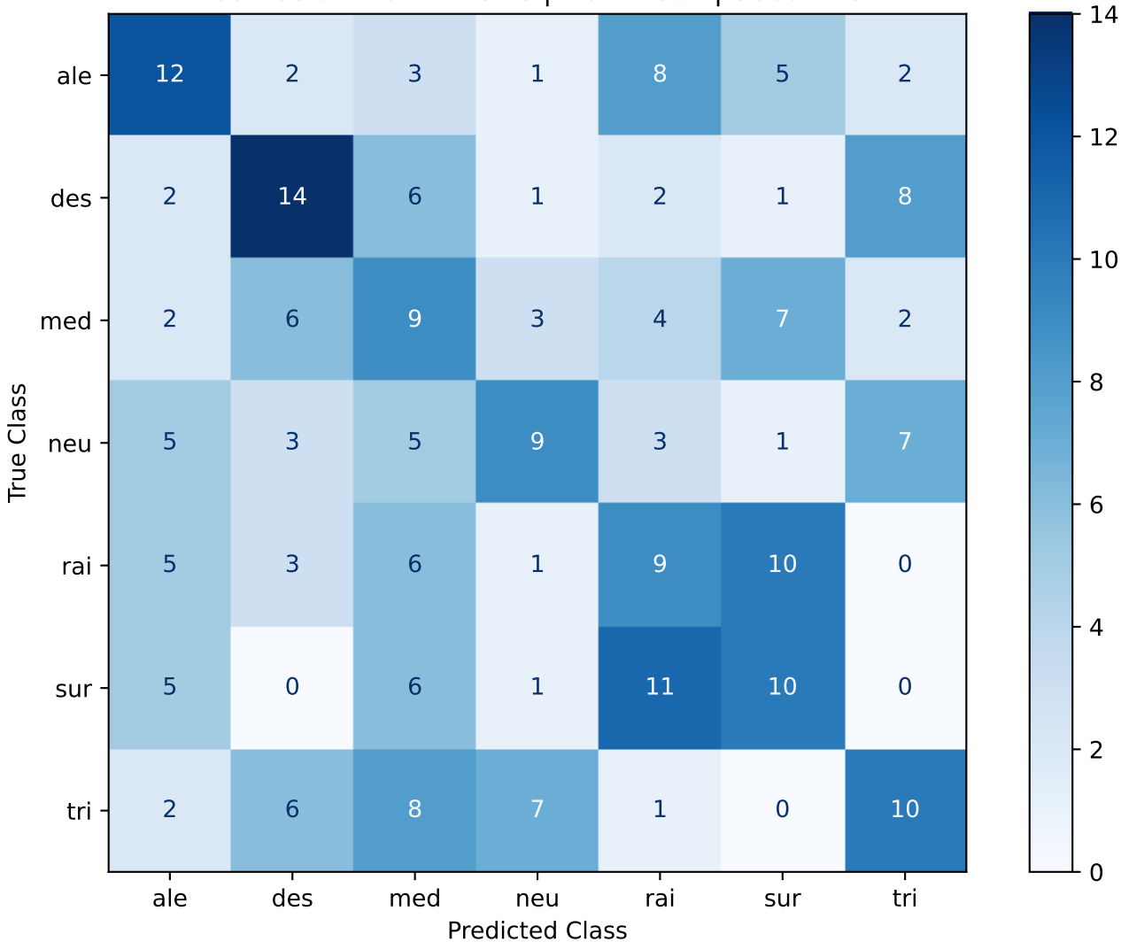
Confusion Matrix - SVC | wav2vec2 | Seed 123
