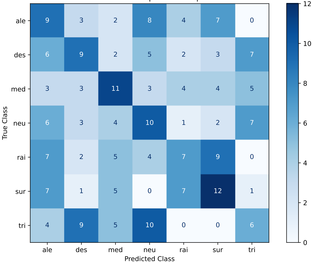
Confusion Matrix - SVC | wav2vec2 | Seed 2025
