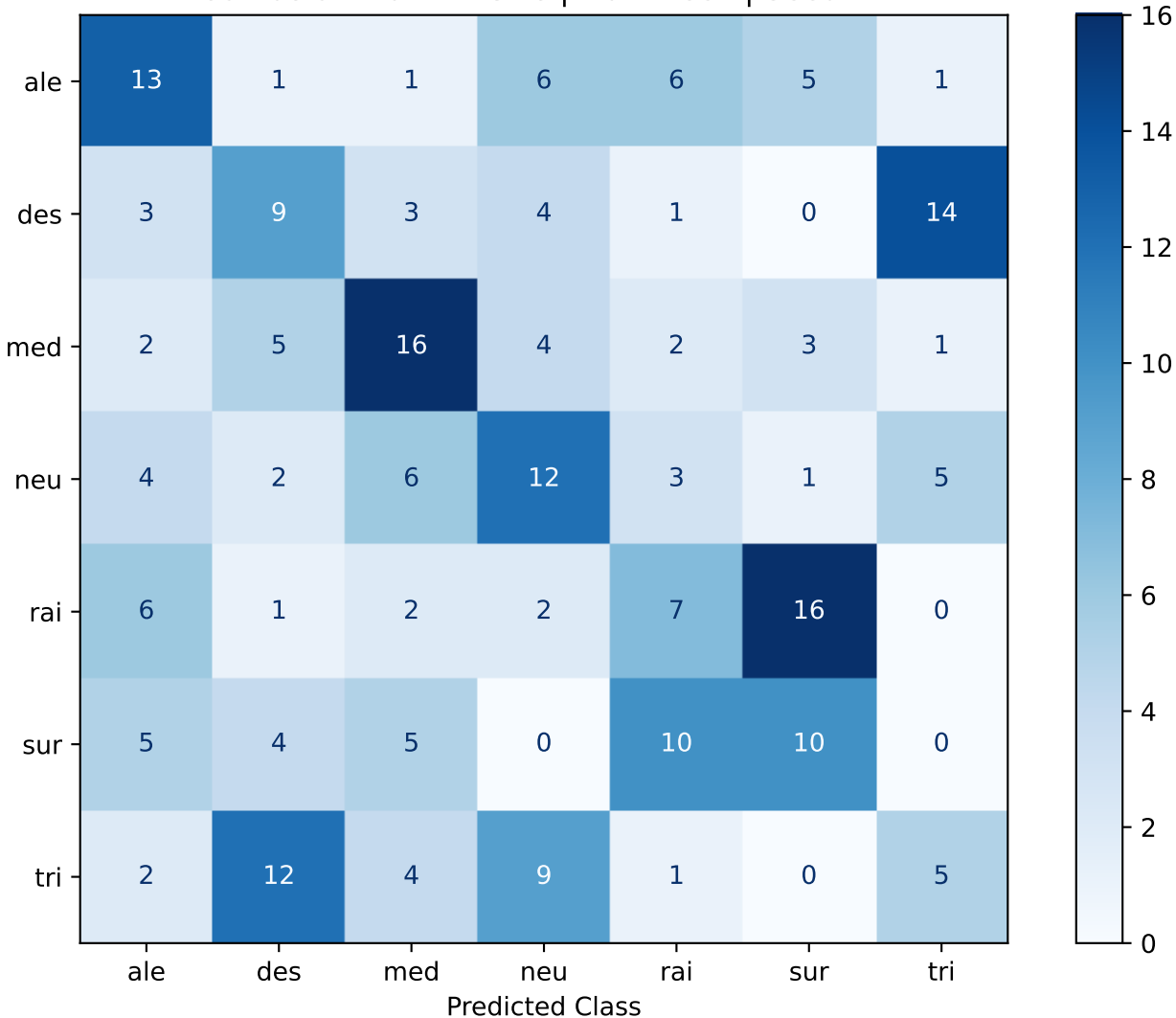
Confusion Matrix - SVC | wav2vec2 | Seed 42
