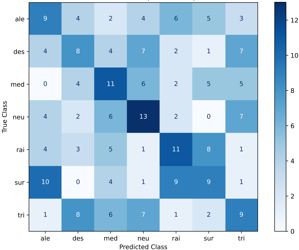
Confusion Matrix - SVC | wav2vec2 | Seed 97
