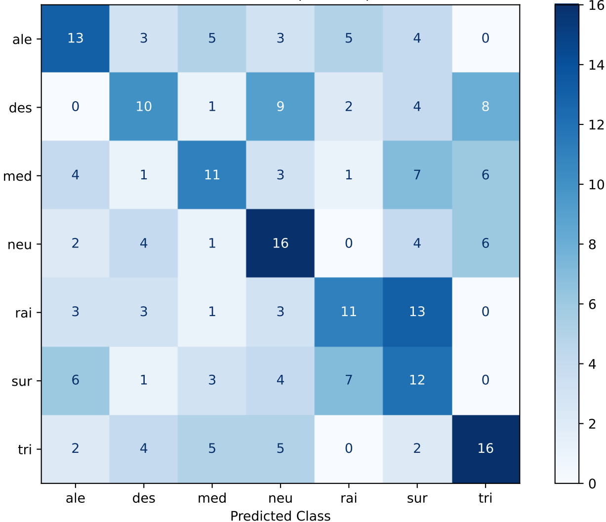
Confusion Matrix - SVC | wavlm | Seed 123
