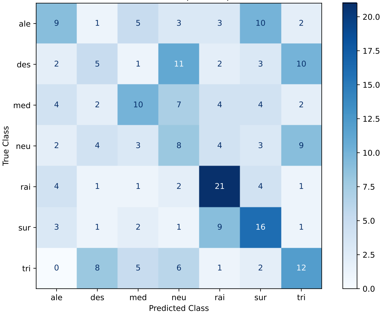
Confusion Matrix - SVC | wavlm | Seed 2025
