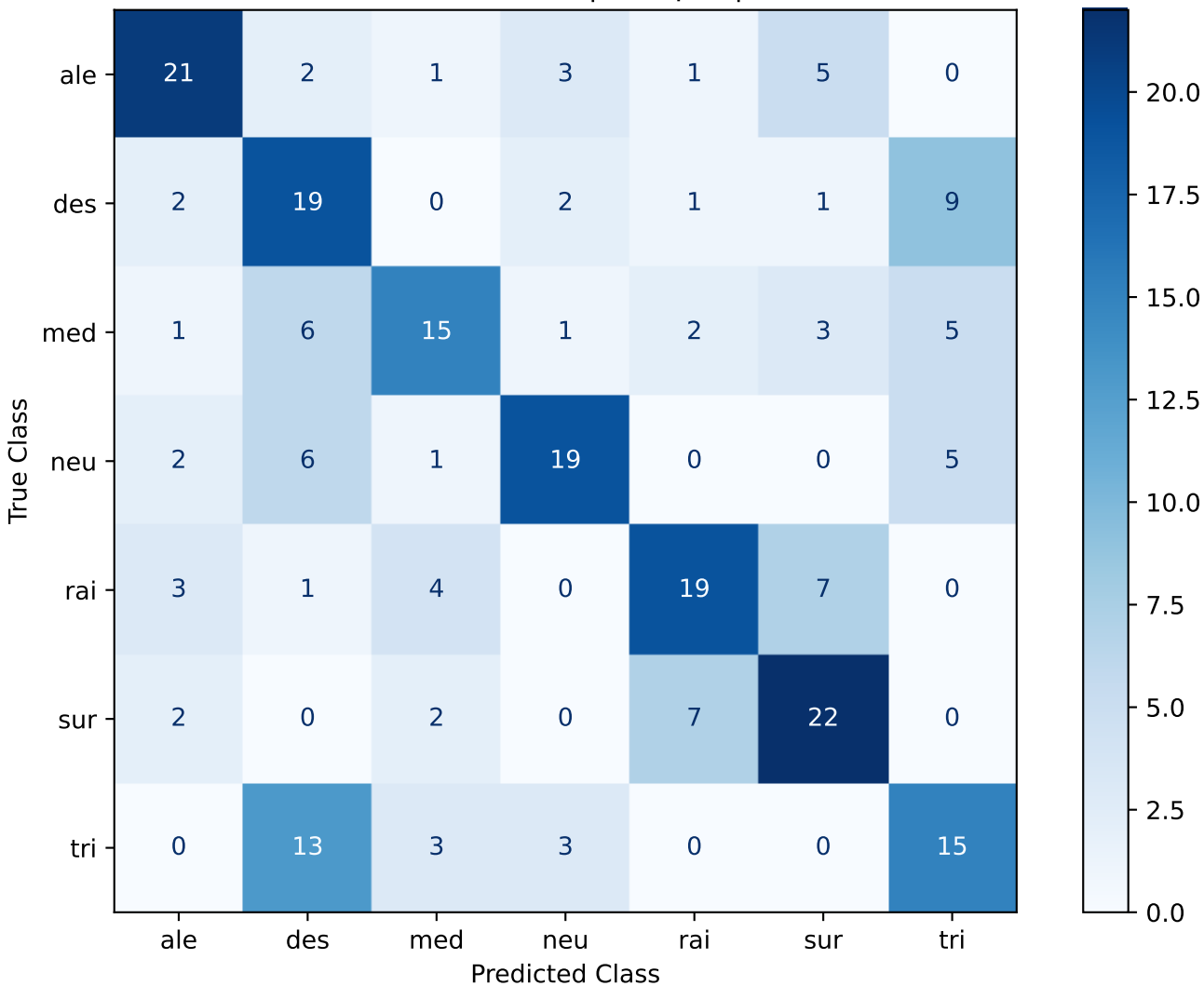
Confusion Matrix - SVC | whisper | Seed 123
