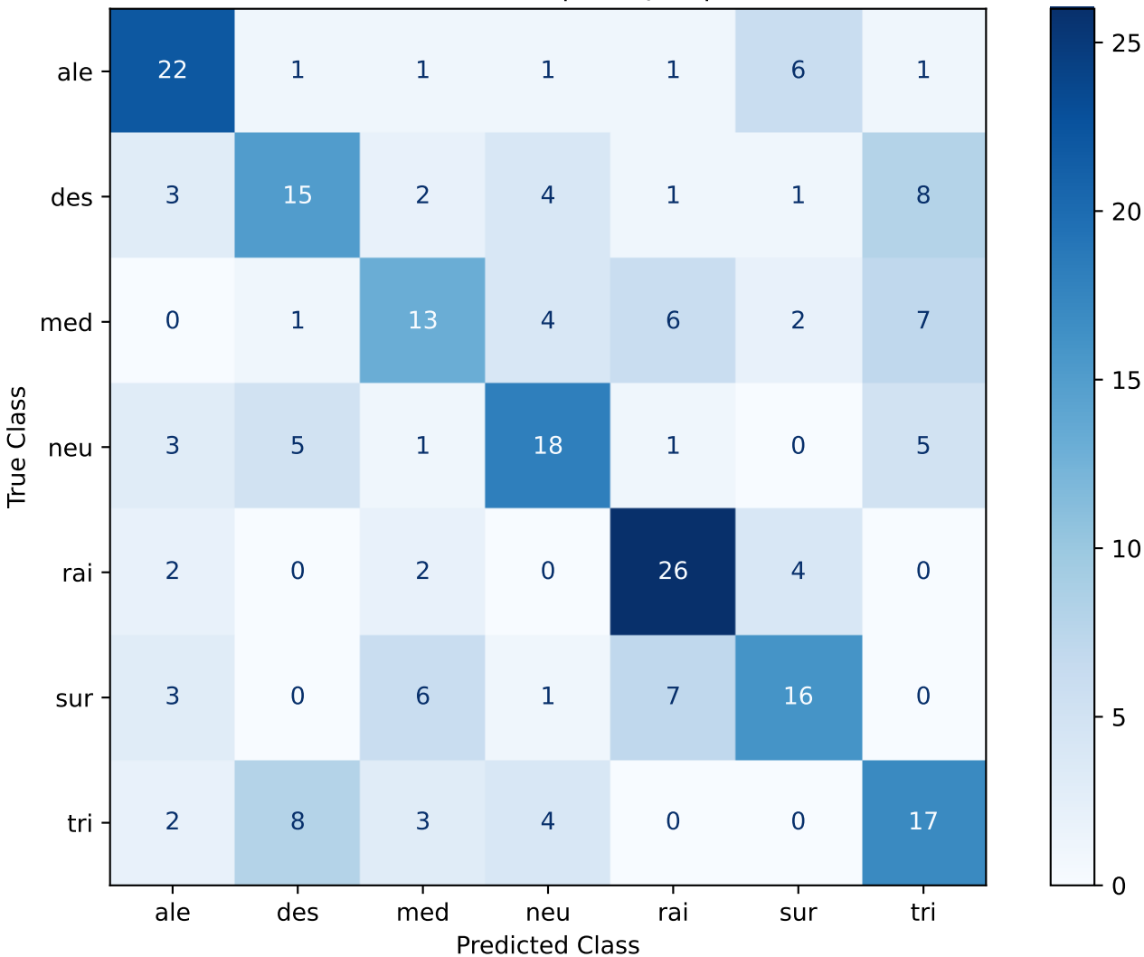
Confusion Matrix - SVC | whisper | Seed 2025
