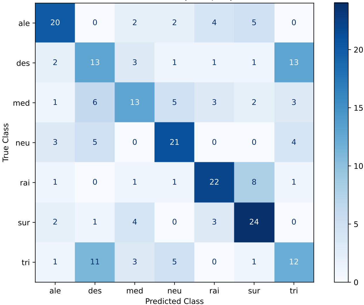
Confusion Matrix - SVC | whisper | Seed 42
