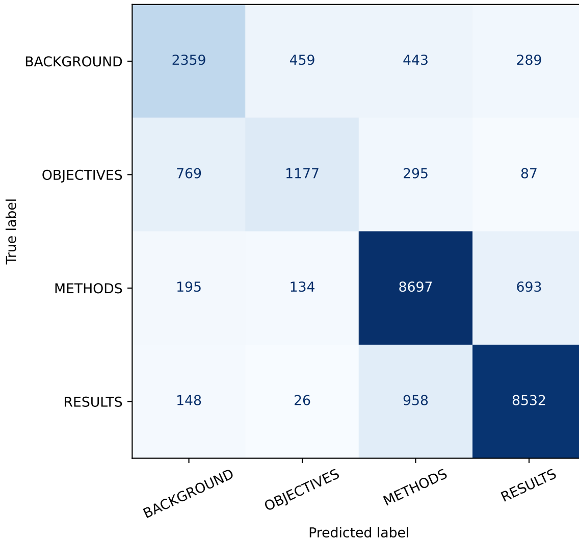
TF-IDF + Linear SVM: Four-Class Test Results
