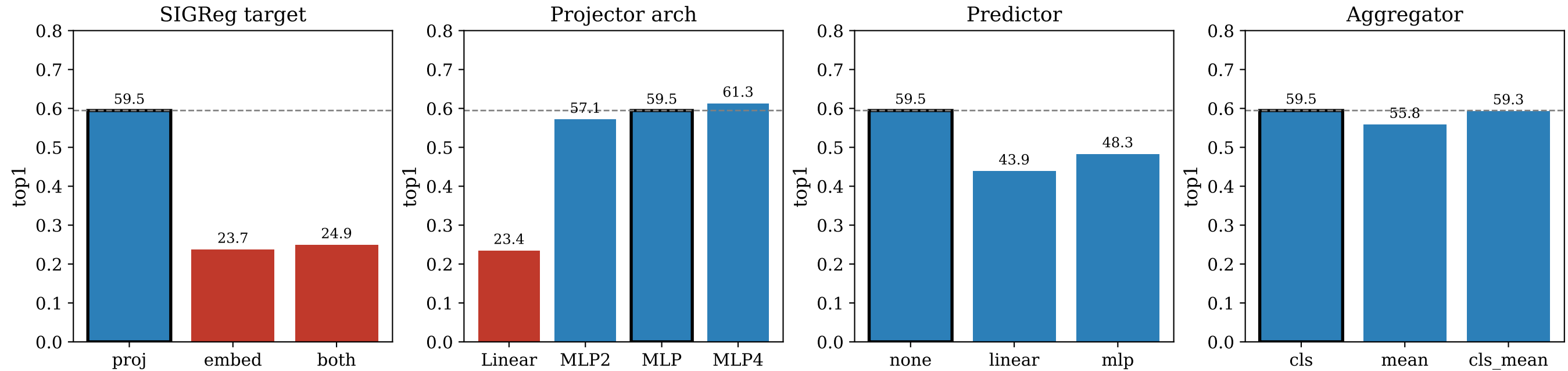
(B) Architecture components — top1 (%). Red = collapse; black edge = baseline; dashed = baseline top1
