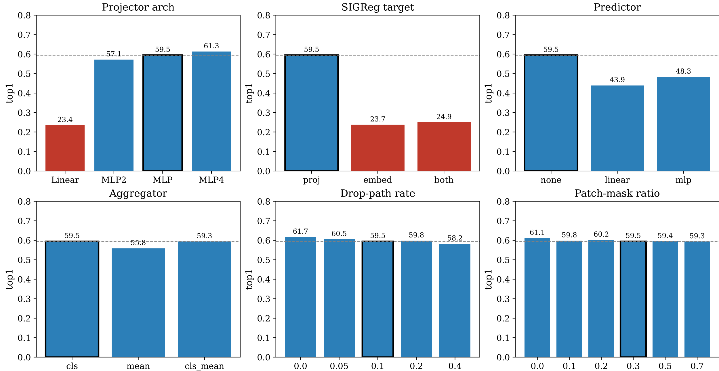
(c) Components & regularizers — top1 (%). Red = collapse; black edge = baseline; dashed = baseline top1
