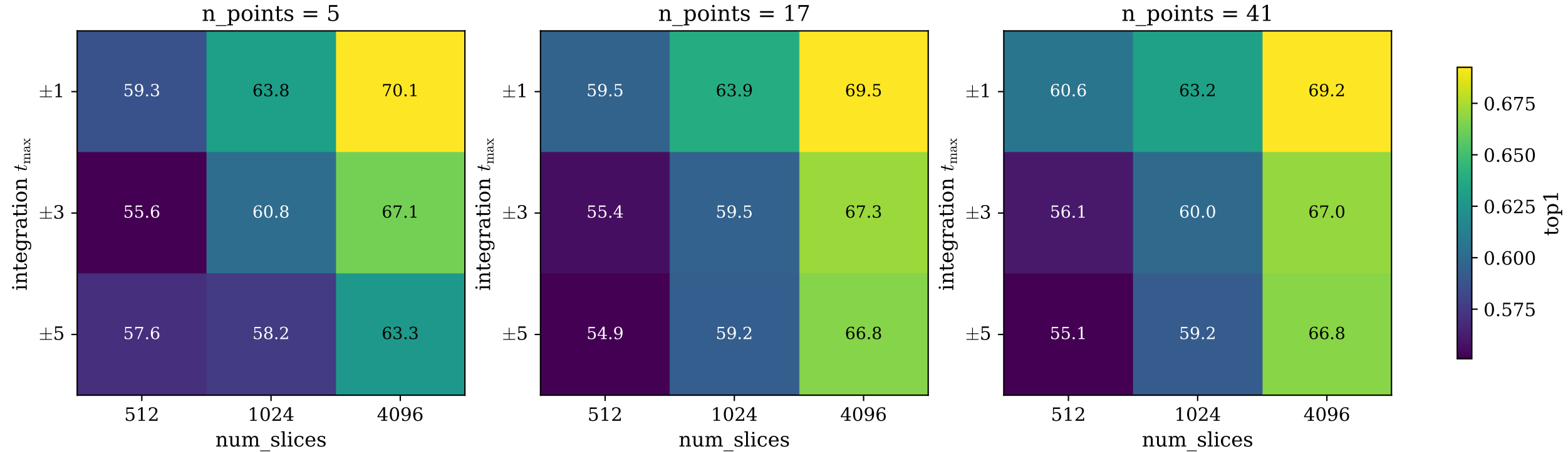
(a) Epps-Pulley integration grid — top1 (%) [ViT-S/16, imagenet10]
