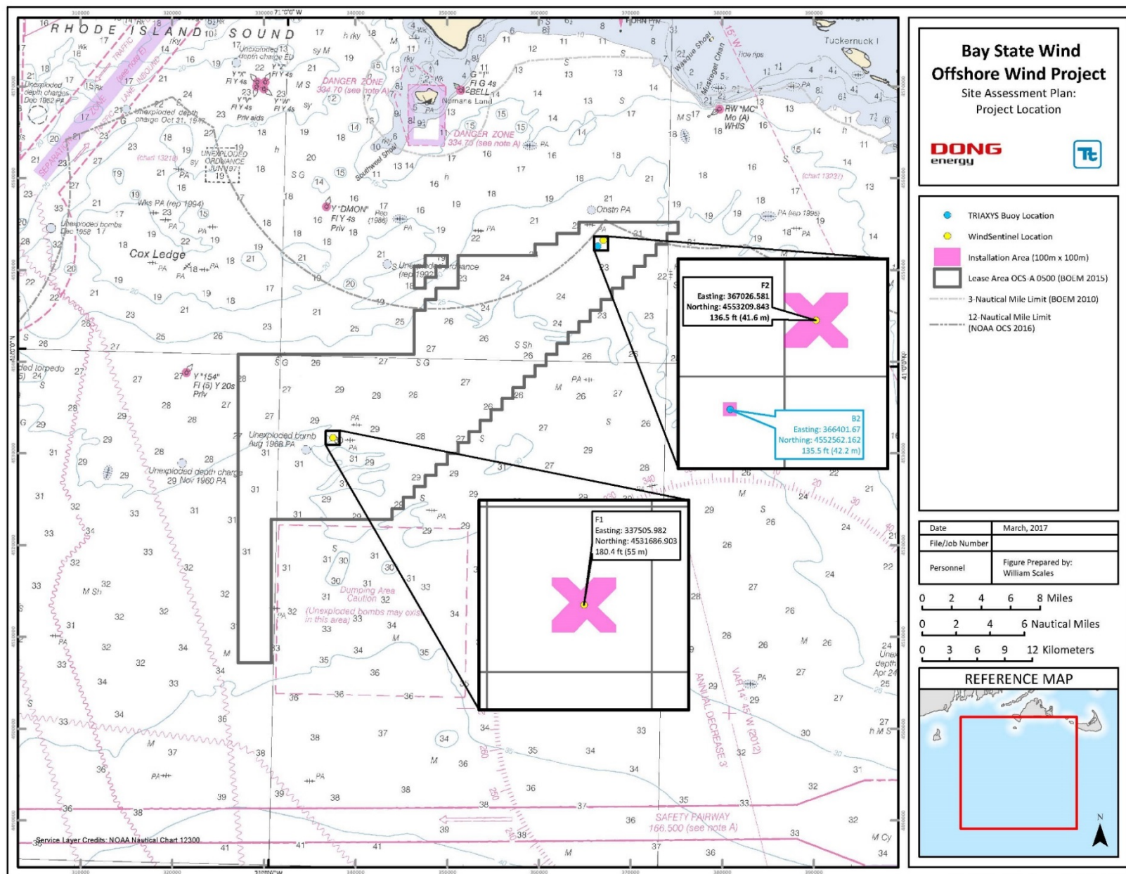
Figure 1-1 Site Assessment Plan Met Buoy Installation Area
