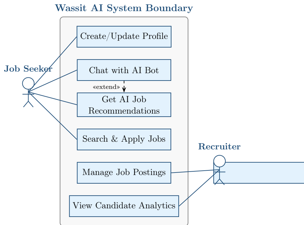
Figure 1: Wassit AI Use Case Diagram
