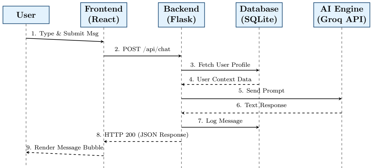
Figure 3: AI Chat Execution Flow Sequence
