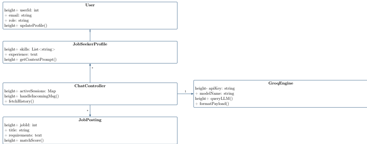
Figure 2: Wassit AI System Structural Class Diagram
