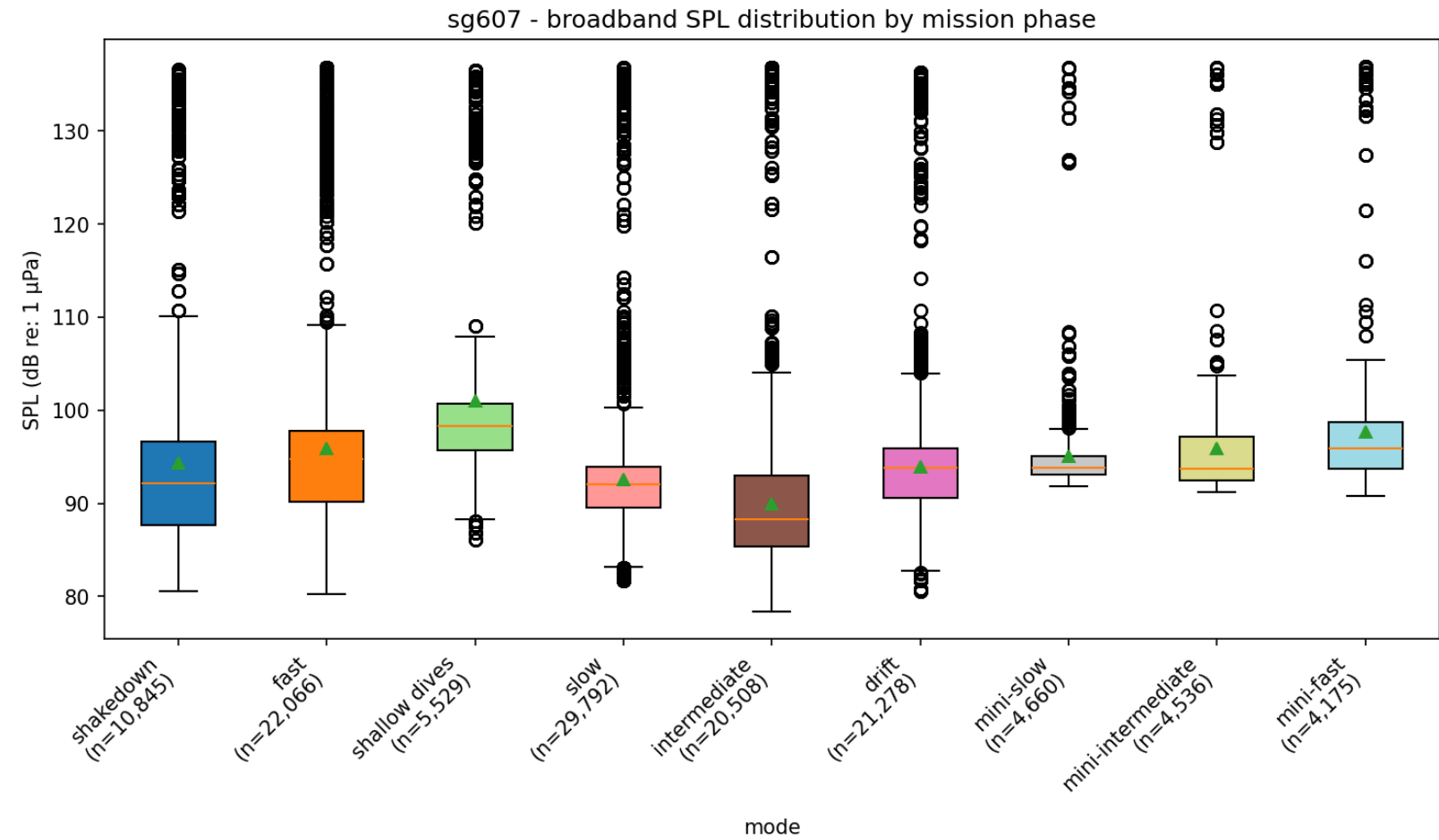
Distribution of broadband SPL for each mission phase.
