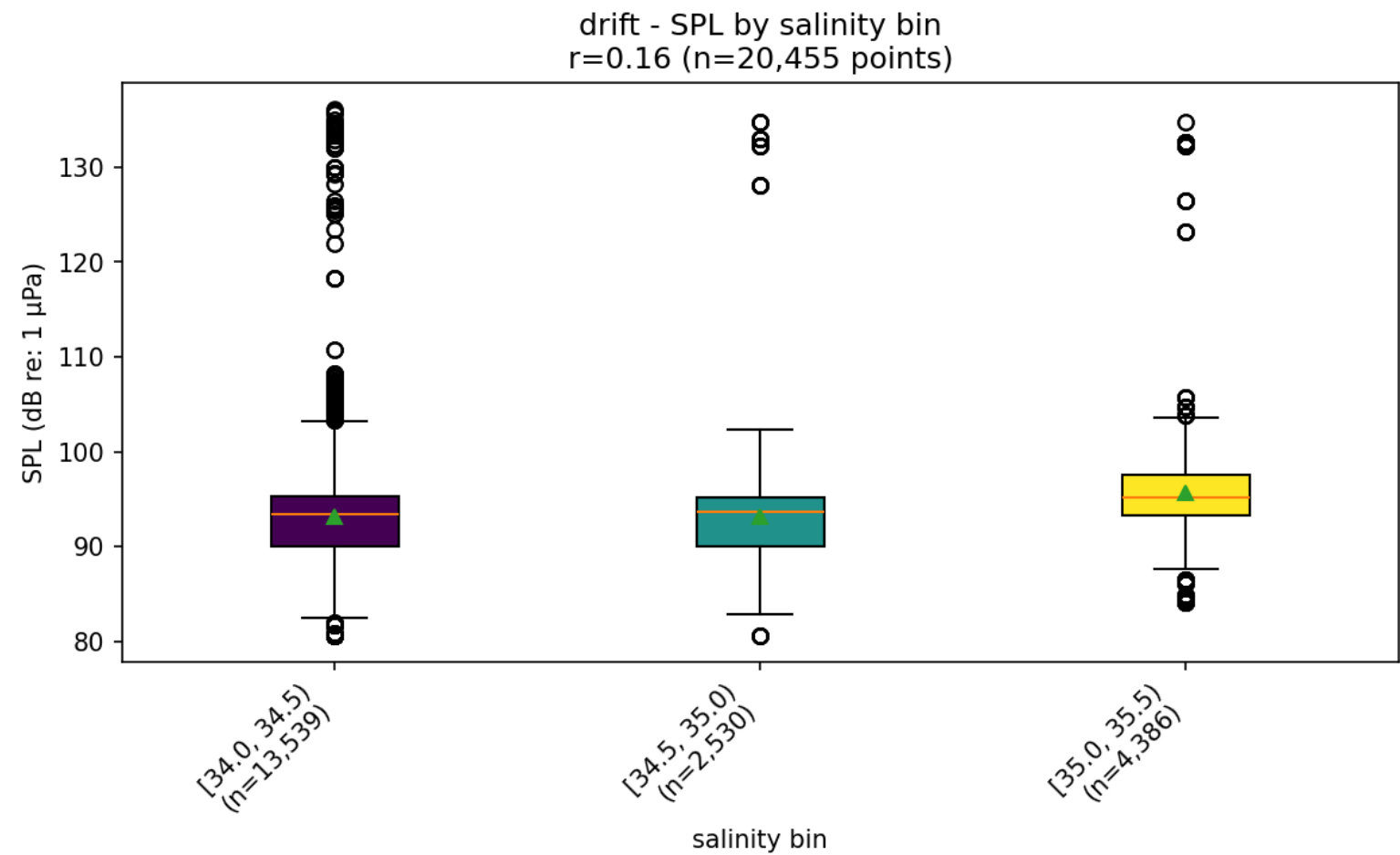
Broadband SPL distribution during "drift", split by salinity bin. Title shows the real per-point Pearson r between raw salinity and raw SPL for this mode.
