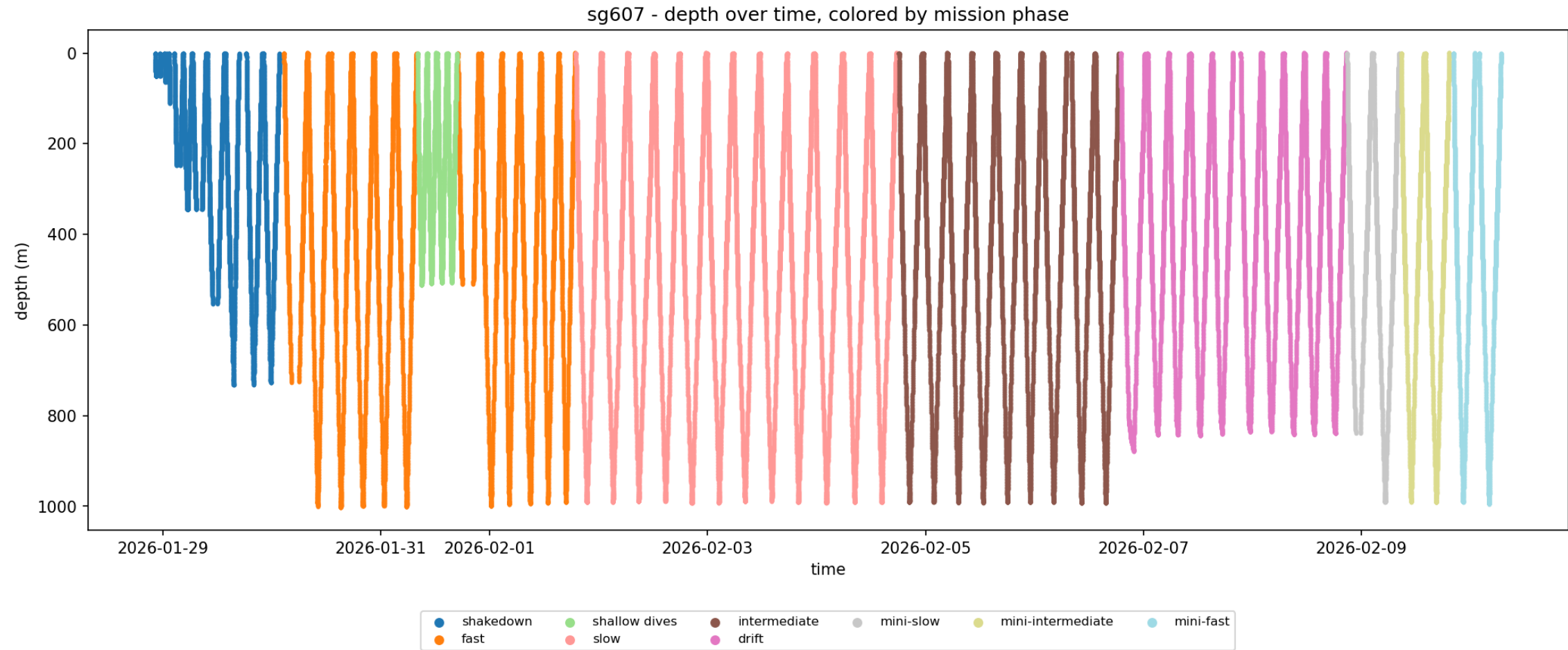
Full-deployment dive profile, colored by mission phase.
