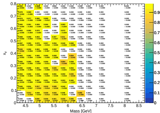
RS62 Avg Hodo Eff (Mix) (LH2)
