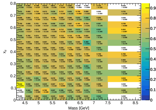
RS62 Avg Signal Efficiency (LH2)
