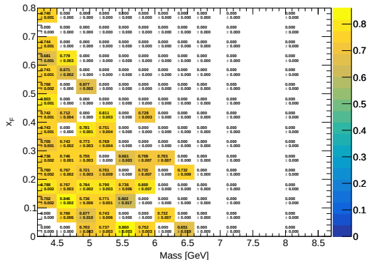
RS67 Avg Hodo Eff (Mix) (Flask)
