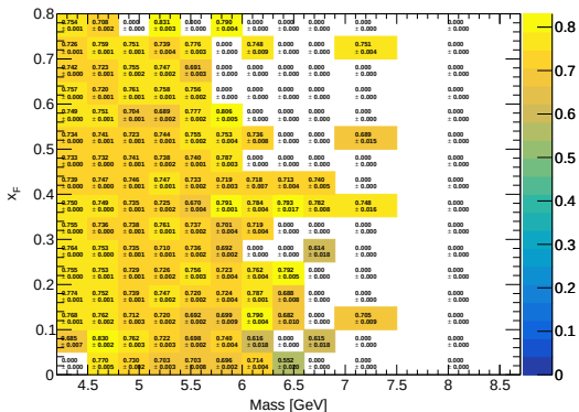
RS67 Avg Hodo Eff (Mix) (LD2)
