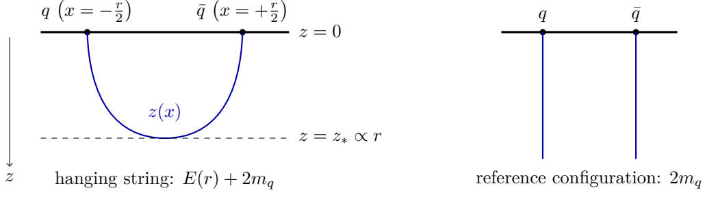
Figure 17.2: The holographic rectangular Wilson loop, in the Poincaré coordinates of (10.11) with the boundary at z = 0 and one spatial direction x shown. Left: the fundamental string ends on the quark and antiquark worldlines at the boundary and sags into the bulk down to the turning point z_* \propto r ; its regularized area gives E(r) in (17.20). Right: the reference configuration of two straight strings falling into the bulk, whose divergent action is the self-energy 2m_q of the infinitely heavy quarks.
