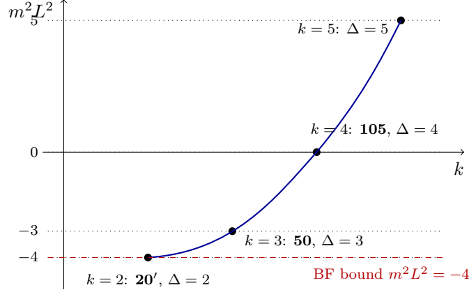
Figure 17.1: The lightest Kaluza–Klein scalar tower on \text{AdS}_5 \times S^5 : m^2 L^2 = k(k-4) in the [0, k, 0] of \text{SO}(6) [80]. The k=2 member saturates the Breitenlohner–Freedman bound; via \Delta(\Delta-4) = m^2 L^2 the tower is dual to the chiral primaries with \Delta = k . Marginal and relevant operators ( \Delta \leq 4 ) correspond to m^2 \leq 0 .
