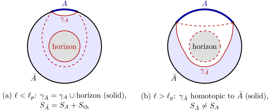
Figure 21.4: The homology rule for the complement \bar{A} of an interval A on a time slice of the one-sided BTZ black hole, with the horizon as inner edge. \gamma_A alone is never admissible for \bar{A} , because the region between them has the horizon as a further boundary. The two admissible surfaces are \gamma_A \cup \text{horizon} and the geodesic homotopic to \bar{A} ; the minimal one is drawn solid, the other dashed, and the shaded region is the homology region of the minimal one. The crossover \ell_p is given in (21.35).
