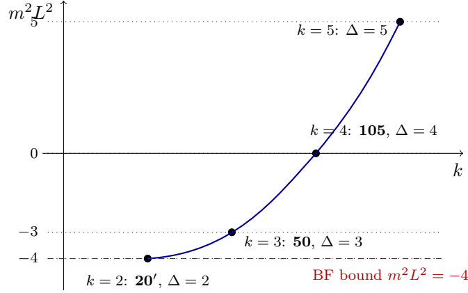
Figure 17.1: The lightest Kaluza–Klein scalar tower on \text{AdS}_5 \times S^5 : m^2 L^2 = k(k-4) in the [0, k, 0] of \text{SO}(6) [82]. The k=2 member saturates the Breitenlohner–Freedman bound; via \Delta(\Delta-4) = m^2 L^2 the tower is dual to the chiral primaries with \Delta = k . Marginal and relevant operators ( \Delta \leq 4 ) correspond to m^2 \leq 0 .
