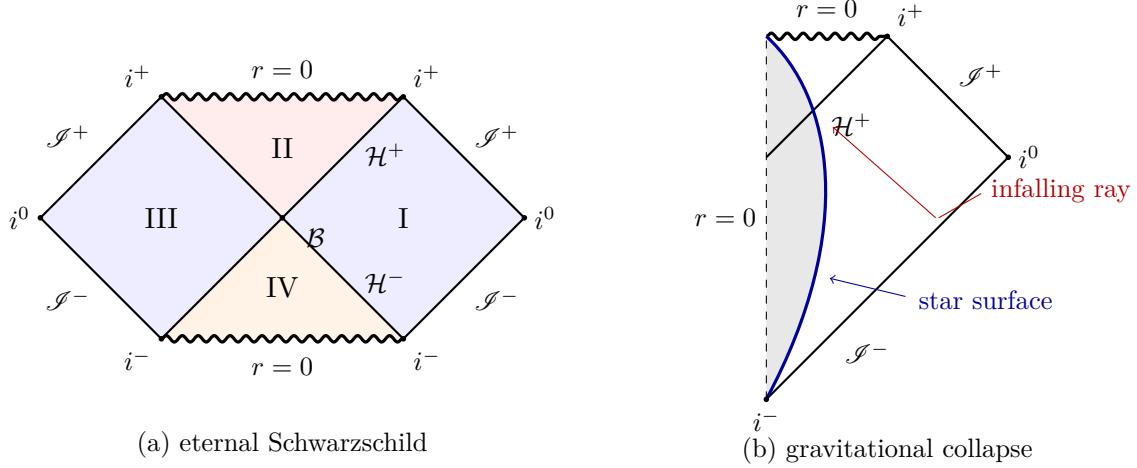
Figure 1.2: Penrose diagrams of Schwarzschild. (a) The eternal, maximally extended solution: two asymptotically flat exteriors I and III share a black hole interior II and a white hole interior IV; \mathcal{B} is the bifurcation sphere, and no causal curve connects I to III. (b) Gravitational collapse: the shaded region is the interior of the star, outside which the geometry is exactly Schwarzschild by Birkhoff's theorem. There is a single exterior, a single future horizon and a single spacelike singularity: no white hole and no second universe. The horizon is generated by the outgoing rays that just fail to escape.
