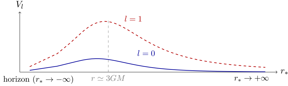
Figure 5.1: The Regge–Wheeler potential (??) for a massless scalar in the Schwarzschild geometry, drawn to scale in units GM = 1 . Even the s-wave sees a barrier; for higher l the barrier peaks near the photon sphere r = 3GM .
