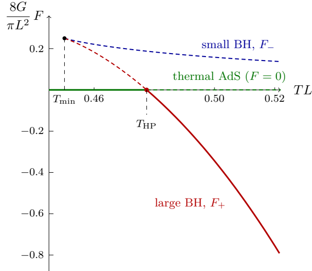
Figure 18.2: The free energies F_{\pm}(T) of (??) for d = 4 , in units of \pi L^2/8G , relative to thermal AdS ( F = 0 at leading order in G ). The two black hole branches emerge in a cusp at T_{\min}L = \sqrt{2}/\pi \simeq 0.450 , where F = \frac{1}{4} in these units. Both decrease with T . The small branch is never dominant. The large branch crosses F = 0 at T_{\text{HP}}L = 3/2\pi \simeq 0.477 and dominates above it. Solid lines mark the dominant phase at each temperature; the kink at T_{\text{HP}} is the first-order transition.
