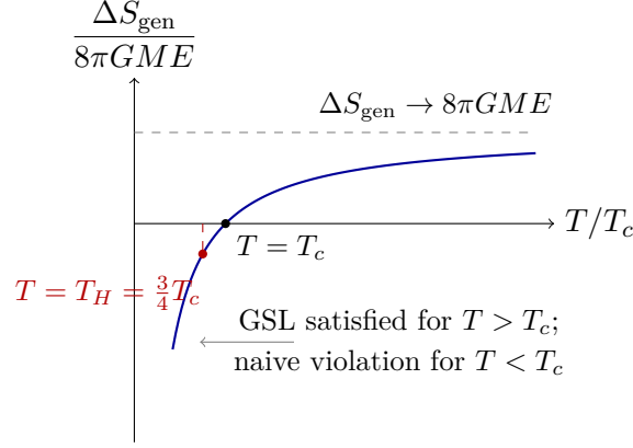
Figure 2.2: The entropy balance (??) for absorption of black-body radiation at temperature T , in units of T_c = 1/6\pi GM . For T < T_c the naive generalized entropy decreases. The Hawking temperature T_H = \frac{3}{4}T_c sits inside the problematic region: the resolution requires the black hole’s own emission.
