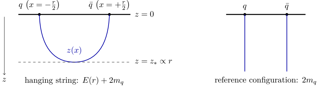
Figure 17.2: The holographic rectangular Wilson loop, in the Poincaré coordinates of (??) with the boundary at z = 0 and one spatial direction x shown. Left: the fundamental string ends on the quark and antiquark worldlines at the boundary and sags into the bulk down to the turning point z_* \propto r ; its regularized area gives E(r) in (??). Right: the reference configuration of two straight strings falling into the bulk, whose divergent action is the self-energy 2m_q of the infinitely heavy quarks.
