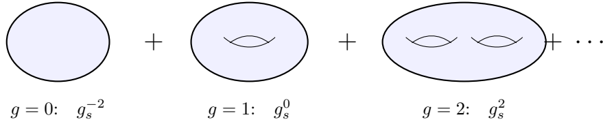
Figure 15.1: Closed-string perturbation theory as a genus expansion (??): one surface of genus g , weighted by g_s^{2g-2} , replaces the Feynman diagrams of a field theory at each loop order. This is the topological expansion of large- N gauge theory in Chapter ??, with g_s^2 \leftrightarrow 1/N^2 .
