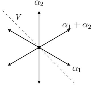
Figure 9: The A_2 root system with positive simple roots \alpha_1, \alpha_2 , and a hyperplane V (dashed) containing no root.
