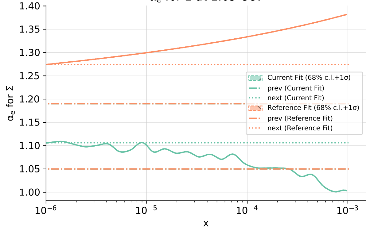
\alpha_e for \Sigma at 1.65 Gev
