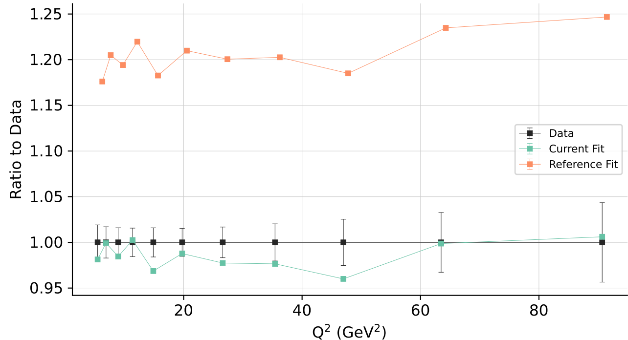
NMC d/p x = 0.275 (shifted)
