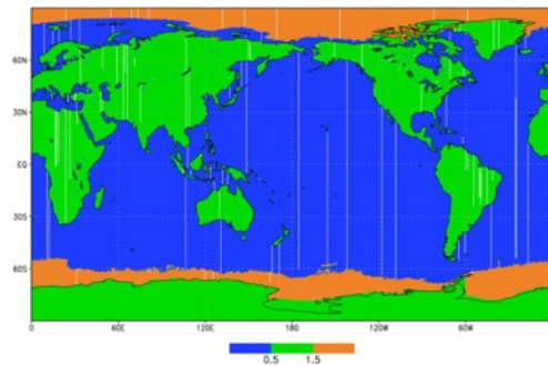
Sea-Land-Ice Mask
