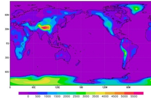
Orography
