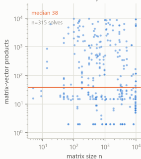
Cost of a successful solve, iterative families only stationary
