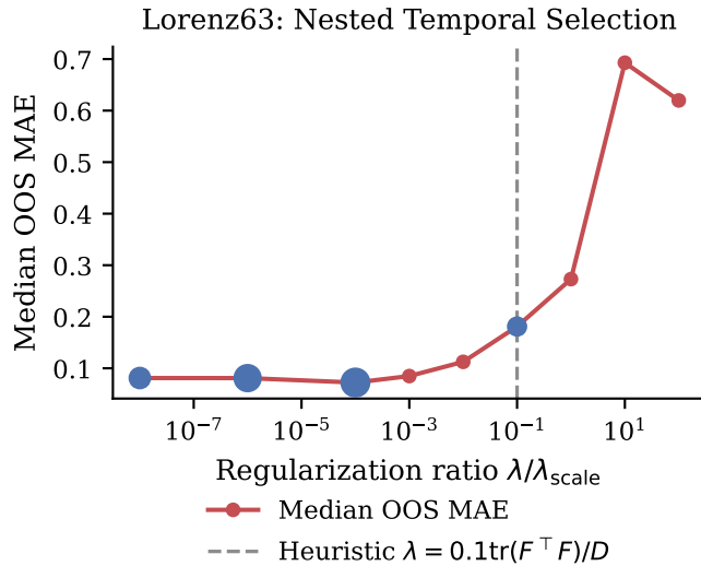
FIG. 4. Nested temporal validation path for the Ridge read-out’s regularization ratio on Lorenz63 (§3 of the main text), showing the internal holdout MAE across the candidate grid and the ratio selected at each outer window.
