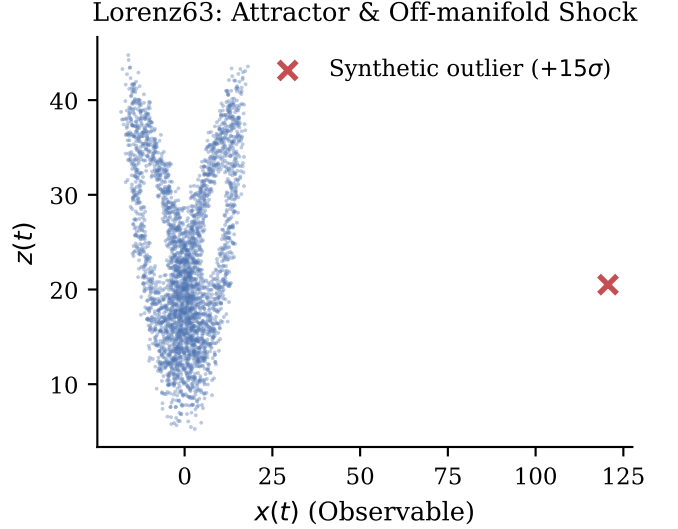
FIG. 2. Phase space reconstruction (x, z) illustrating the excursion of an additive unphysical outlier ( +15\sigma ) outside the low-dimensional fractal attractor manifold of Lorenz63.
