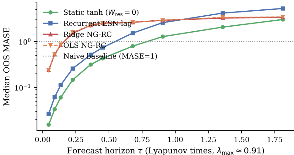
Lorenz63: Iterated Multistep Stability
