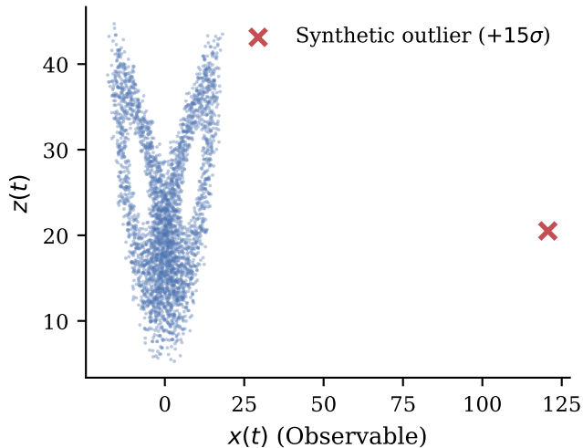
Lorenz63: Attractor & Off-manifold Shock
