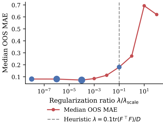
Lorenz63: Nested Temporal Selection
