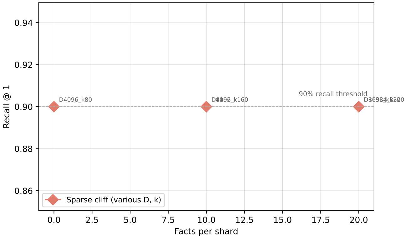
Per-shard capacity: dense bipolar vs. sparse-binary HRR
