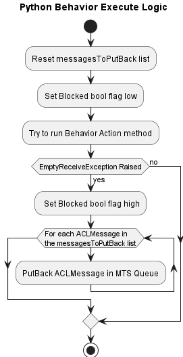
Figure 5.6: Python Behavior Execute Activity Diagram.
