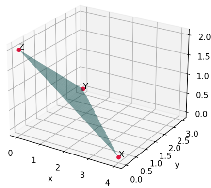
Plane: x/4 + y/3 + z/2 = 1
