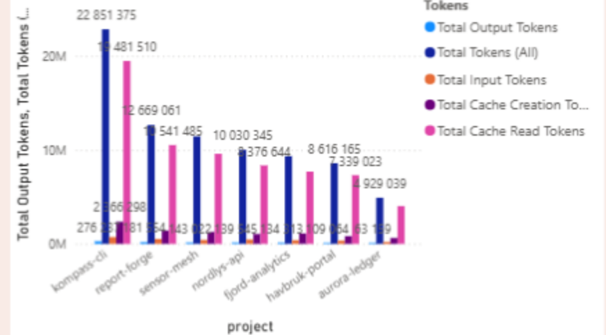
Total Tokens
