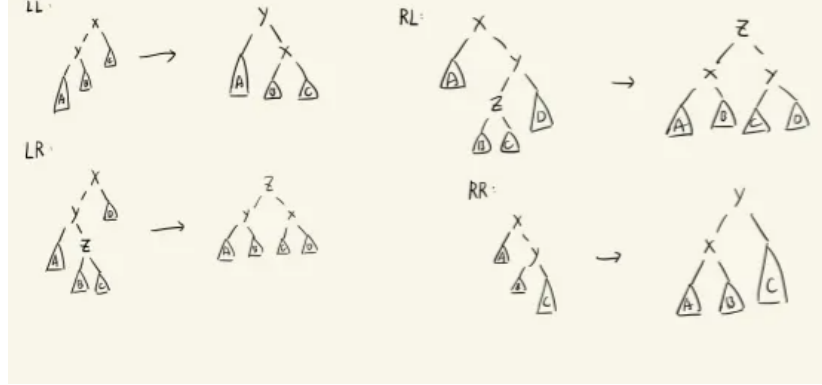
Figure 4: AVL Tree
