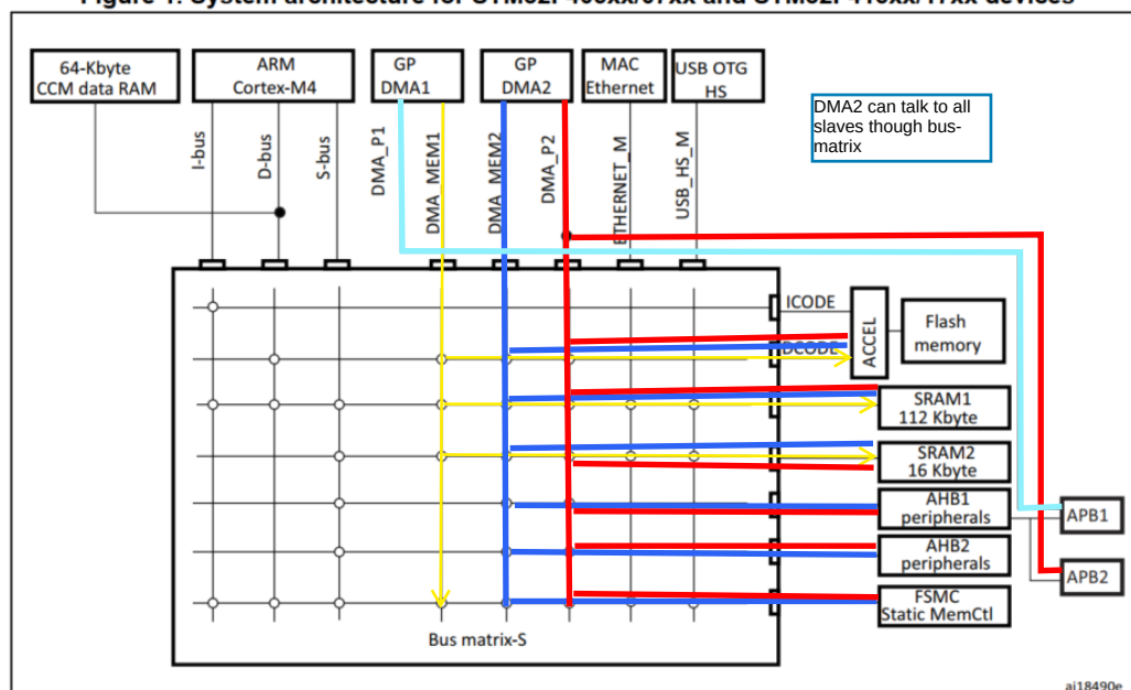
Figure 1. System architecture for STM32F405xx/07xx and STM32F415xx/17xx devices
