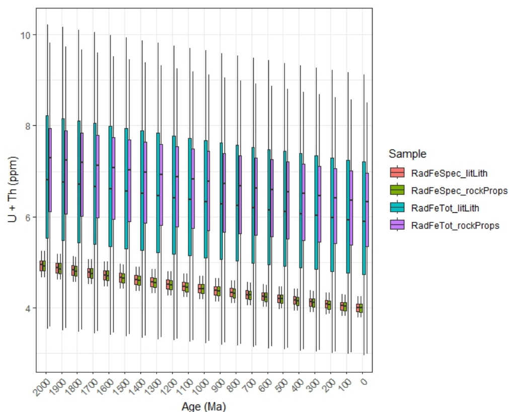
Figure 2: Decay of uranium and thorium over geological time scales, lowering the H_2 and He production rate through radiolysis.
