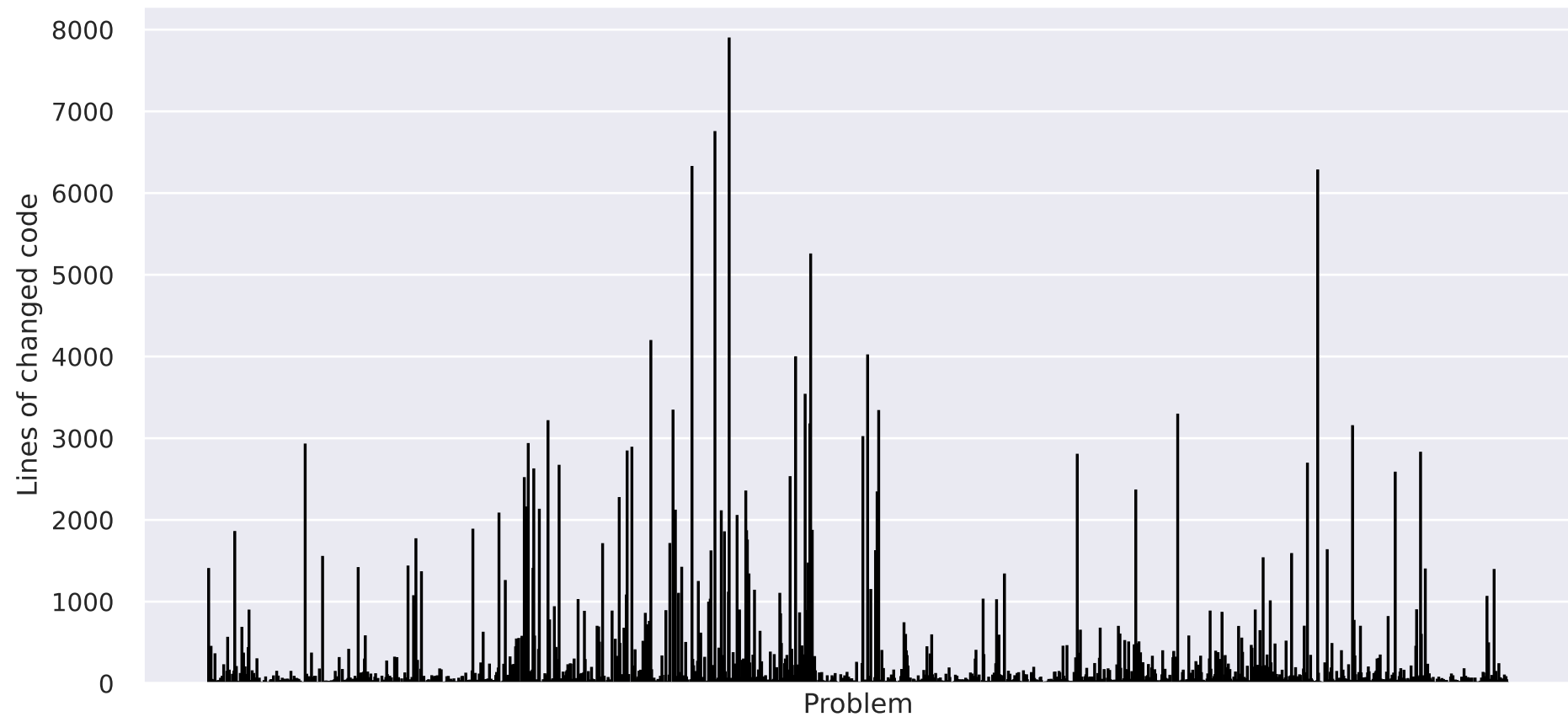
Lines of changed code distribution in issues's patch
