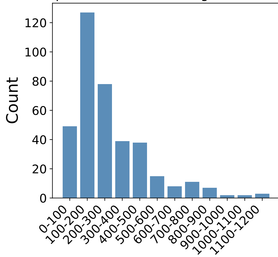
Go problem statement length distribution
