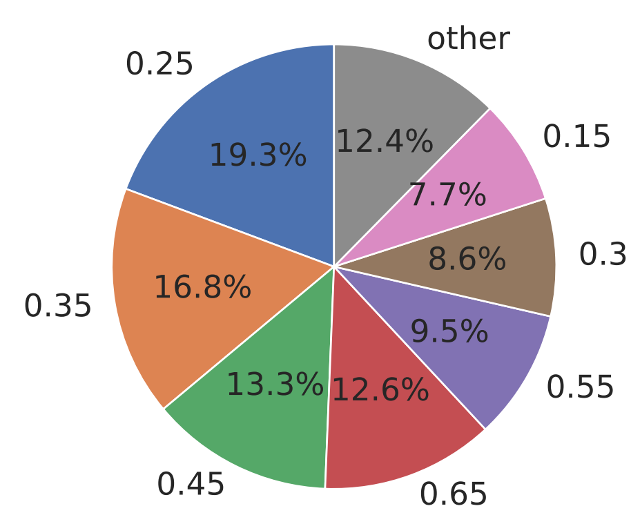
Rust difficulty distribution
