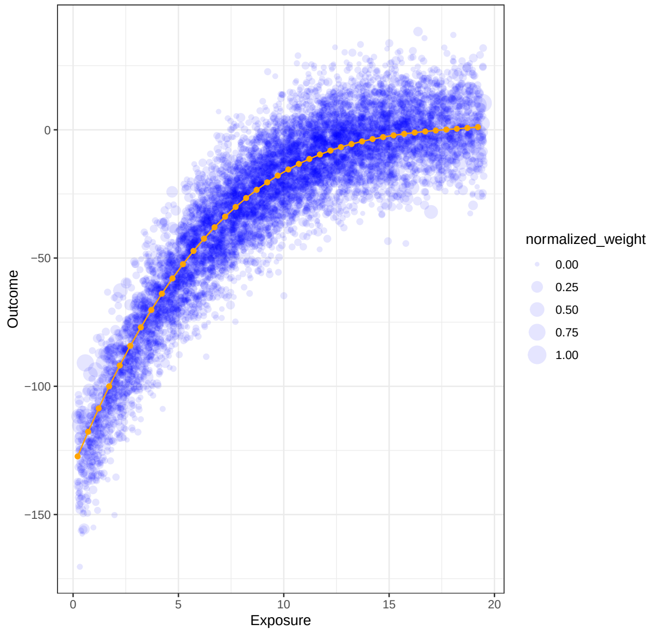
Exposure Response Curve for parametric model
